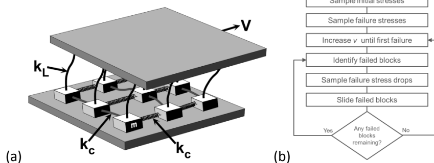
Figure 3.25 Schematic illustration of a simple slider-block model of seismicity on a single fault; adapted from Rundle (2003). (b) Example of simple physical rules that govern the evolution of a slider-block system.
