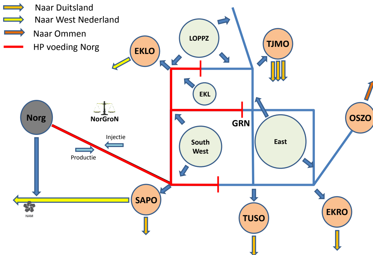
Figure 3.10 Schematic of the Groningen gas ring pipeline system as operated during the summer months with two pressure regimes.
